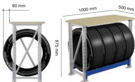
Workbench for tire storage R15 195/65, R16 205/55
